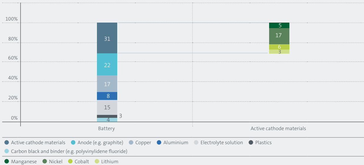
Lithium-ion battery and cathode component distribution by weight, example of an NMC 622 cathode material
